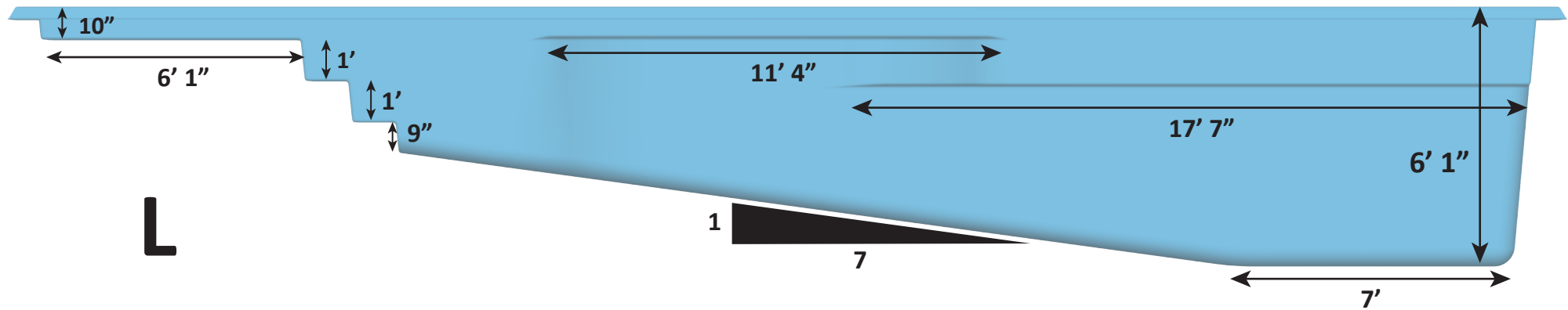
Side View
